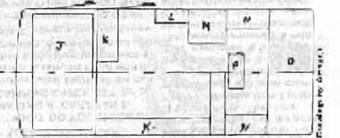
EYE-LEVEL PLAN OF VAN
