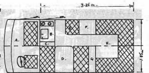
FLOOR PLAN OF VAN
